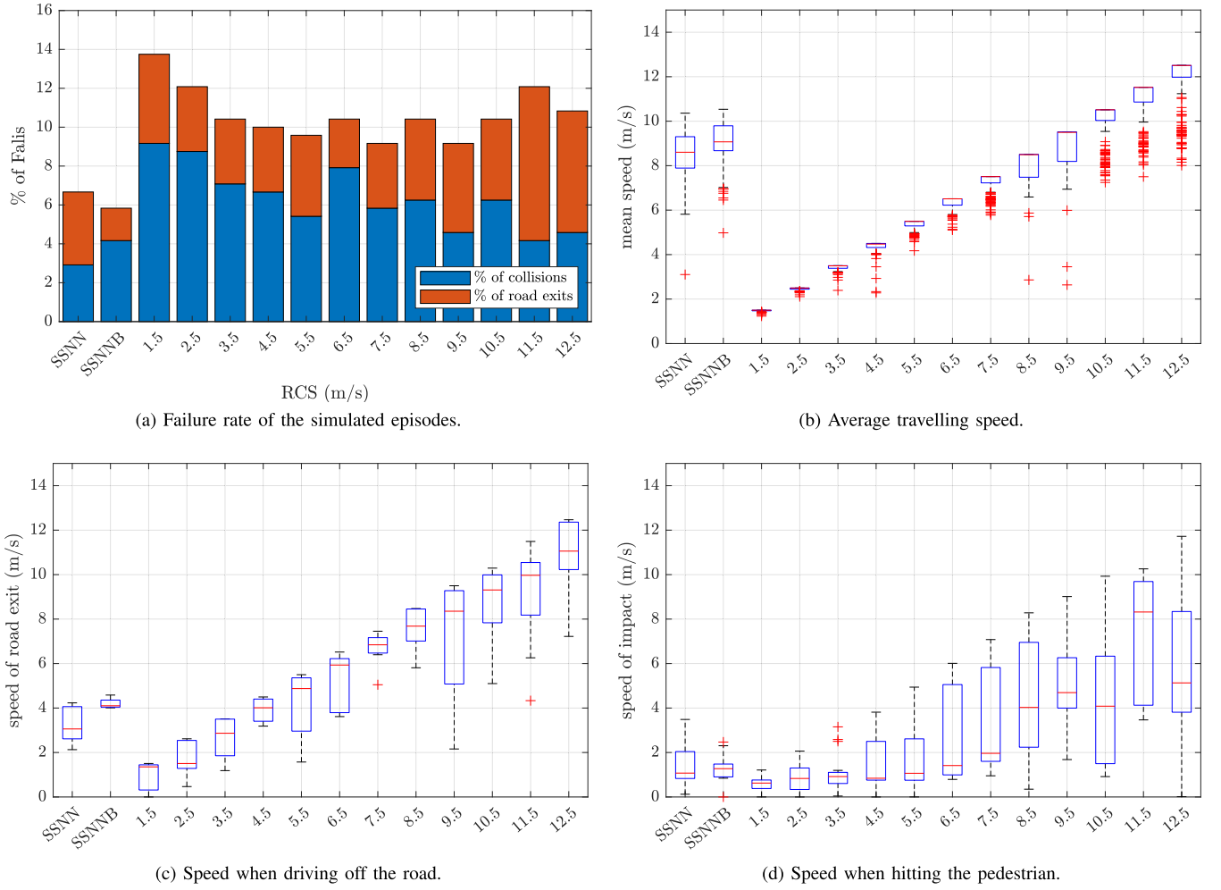
Fig. 11. Statistical evaluation of the performance of the driver agent with or without safe speed network. The leftmost columns of each plot show the ADS performance with the SSNN (the SSNNB refers to a slightly different version of the SSNN described in Section VII-A). The remaining columns show the performance of the ADS without the safe speed network with different posted speed limits.
