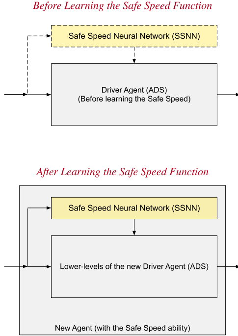
Fig. 3. The learning of a safe speed behavior follows the method used to extend subsumption architectures: a given agent (ADS) is enhanced by developing a new layer (SSNN) that subsumes the original agent’s abilities, resulting in a new agent with extended sensorimotor abilities.
