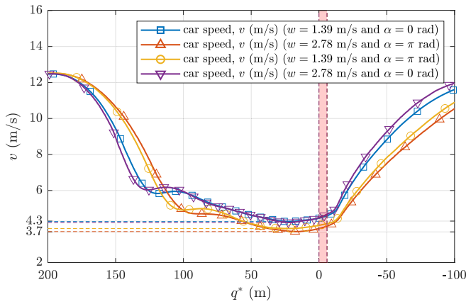
Fig. 10. Results of the integrated framework on four simulations using different constant speed and orientation of the pedestrian. The vertical axis shows the speed of the vehicle (m/s), highlighting its minimum values in the four simulations. The horizontal axis shows the longitudinal displacement of the pedestrian (m), highlighting in red the area of possible collision (-2 * (\frac{L+R}{2} + \delta) \leq q^* \leq 0) .
