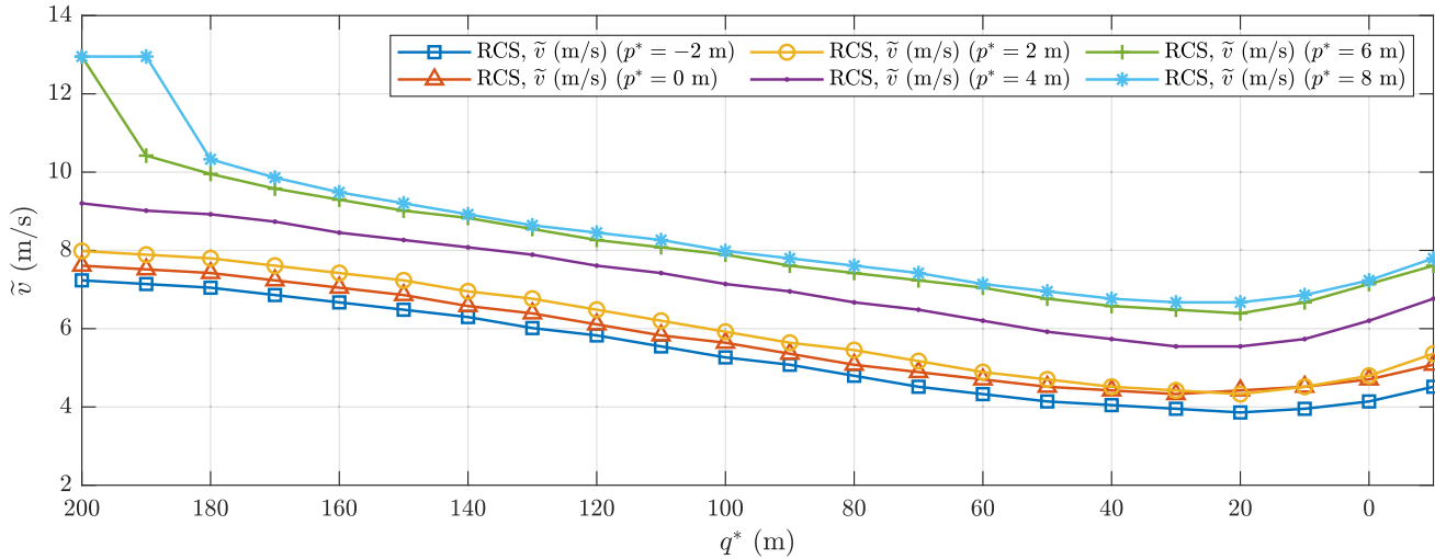
Fig. 13. The RCS suggested by the SSNNB algorithm for different lateral displacement, p^* when the pedestrian walks at 1.39 m/s (5 km/h) parallel on the road in the same direction of the ego vehicle.
