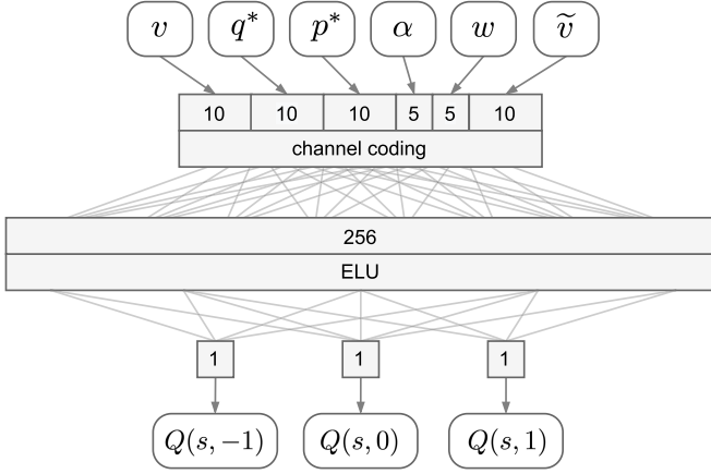
Fig. 5. Architecture of the SSNN.
