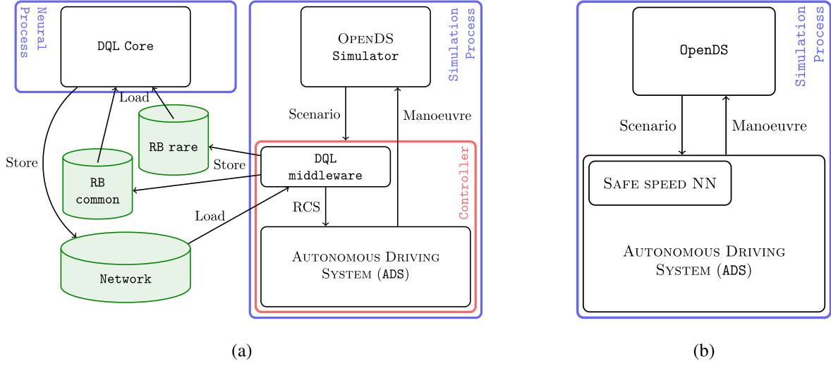
Fig. 7. Framework of integration between the autonomous driving system and the safe speed neural network, for the training phase (a) and for the inference phase (b), i.e. the use of the trained network.
