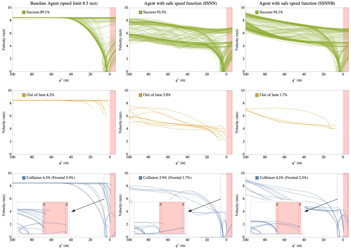
Fig. 15. Comparison between the baseline agent (the driver agent without safe speed function) at 8.5 m/s, agent with the SSNN network, and the agent with the SSNNB algorithm. The three have almost the same mean speed, but the agents with a safe speed network modulate the speed limit getting fewer and less severe failures. Detailed comments are given in the text.
