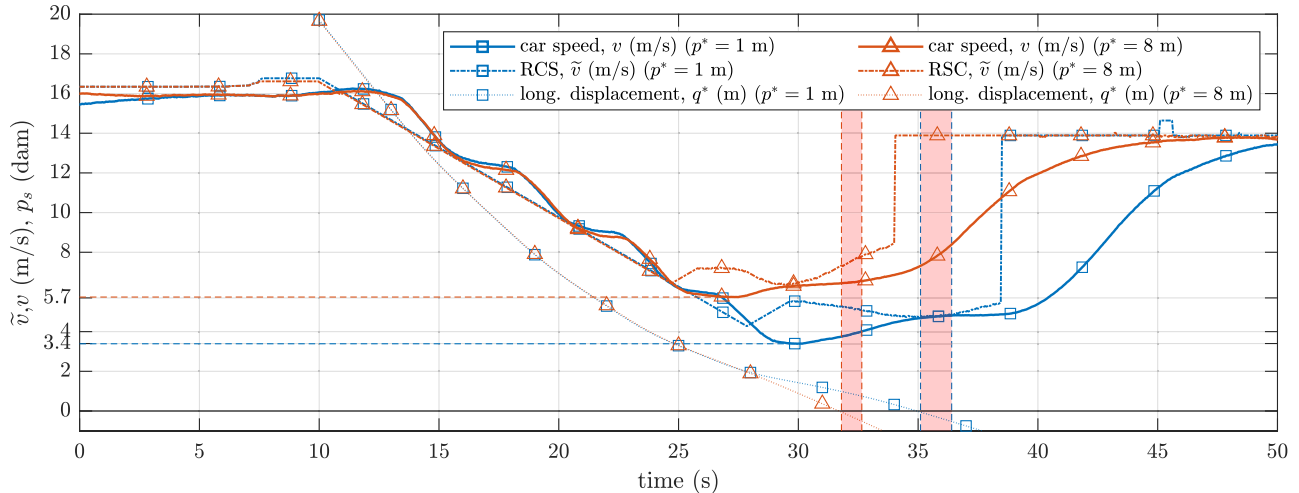
Fig. 12. Results of the integrated framework on two experiment on a real vehicle using different constant lateral displacement of the pedestrian. Each simulation is indicated using the same color and line marker. While the different line style highlights the different variables. The vertical axis shows: the longitudinal displacement (dam), the RCS, \tilde{v} (m/s), and the speed of the vehicle, v (m/s) highlighting its minimum values in the three simulations. The horizontal axis shows the time of simulation (s). The red bands represent the area of possible collision (-2(\frac{L+R}{2} + \delta) \leq q^* \leq 0) .
