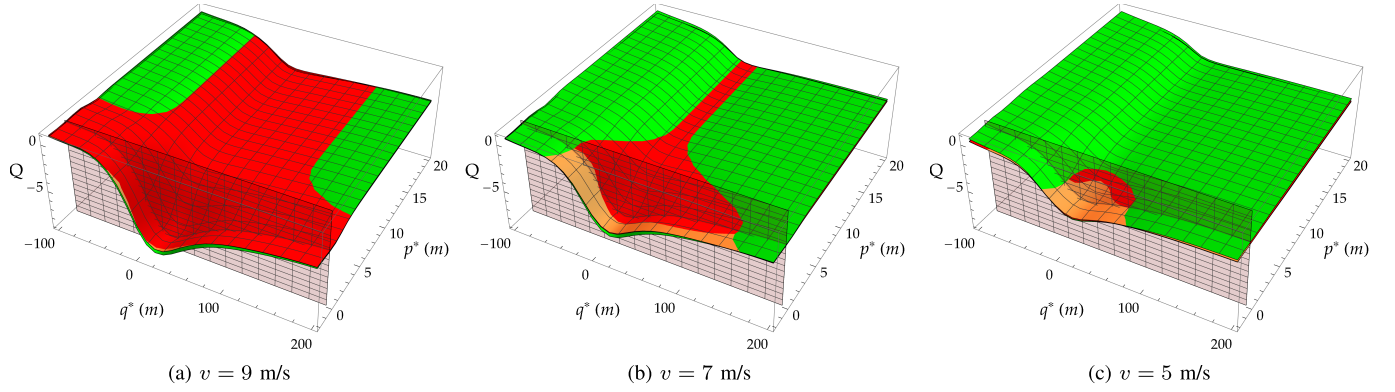
Fig. 8. Visualization of the estimated future rewards Q computed by the network for a given set of states, varying the location of the pedestrian q^* , p^* and the speed of the vehicle v . The color of the surfaces represents the corresponding chosen action: increase the RCS in green, decrease the RCS in red, and keep the RCS constant in orange.
