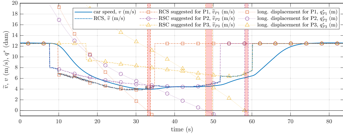
Fig. 14. Results of the integrated system using the SSNNB on a simulation with three pedestrians. P1 (pedestrian 1) advances aligned with the road with speed equal to 2.8 m/s (10 km/h) and lateral displacement, p^* = 2 with direction opposite to that of the ego vehicle. P2 advances aligned to the road with a speed of 1.39 m/s (5 km/h) and lateral displacement, p^* = 2 (opposite side) with the same direction as the ego vehicle. P3 walks perpendicularly away from the road with a speed of 0.14 m/s (0.5 km/h). For each pedestrian, the suggested RCS (dash-dotted line) and the longitudinal displacement (dotted line) are shown with the same color and line marker; for P1 using red squares; for P2 using purple circles; for P3 using yellow triangles. The proposed final RCS, \tilde{v} (m/s) and the speed of the vehicle, v (m/s) are represented in dashed blue and solid blue lines, respectively. The horizontal axis shows the time of simulation (s). The red bands represent the area of possible collision (-2(\frac{L+R}{2} + \delta) \leq q^* \leq 0) .
