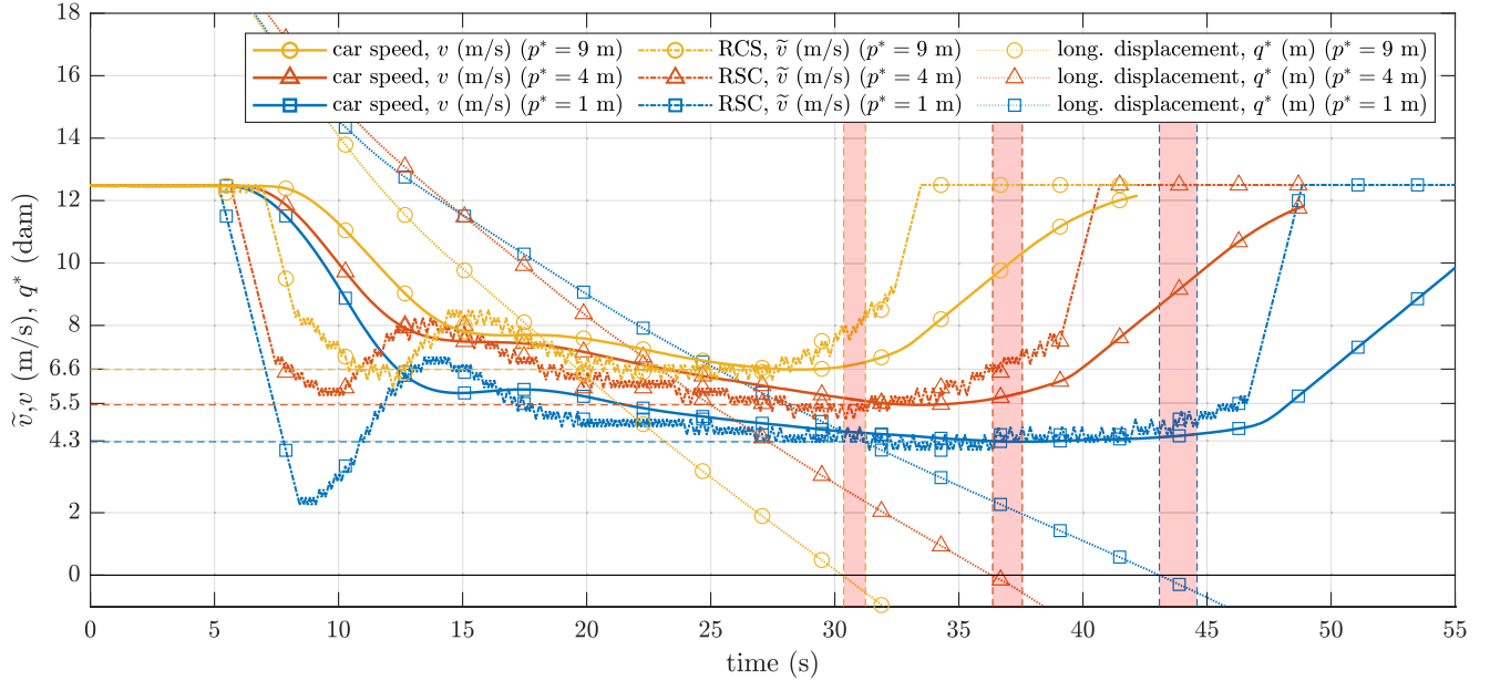
Fig. 9. Results of the integrated system on three simulations with different lateral displacement of the pedestrian. Each simulation is marked with the same color and markers. Different line styles indicate different variables. The vertical axis shows: the longitudinal displacement, q^* (dam), the RCS, \tilde{v} (m/s), and the speed of the vehicle, v (m/s). Note the minimum speed undershoots. The horizontal axis shows the simulation time (s). The red vertical bands represent the areas of possible collision (-2 * (\frac{L+R}{2} + \delta) \leq q^* \leq 0) .
