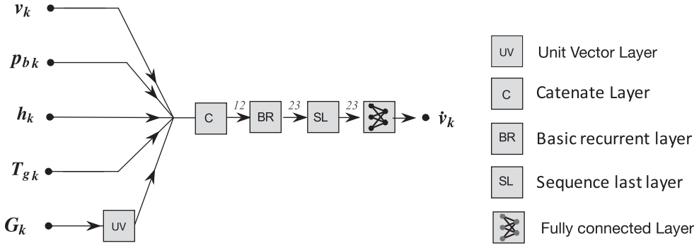
Figure 6. Unstructured recurrent network (iii).
