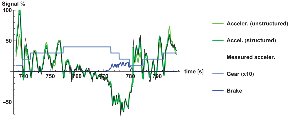
Figure 3. Example of measured signals and convolutional networks prediction. Accelerations are rescaled with respect to the maximum measured acceleration ( 3.1 \text{ ms}^{-2} ).
