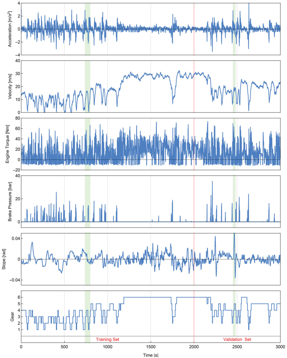
Figure A1. Experimental data. The first part of the data is used as training set and the second part is used as validation set. The green bands refer to the sample intervals used in Figures 3, 10 (in the time range 737 s - 800 s), and 12 (2451 s - 2481 s).
