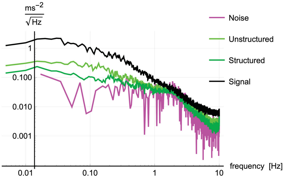
Figure 4. Power spectral density of acceleration measurement noise, convolutional neural networks fit residuals and measured acceleration signals (training set).
