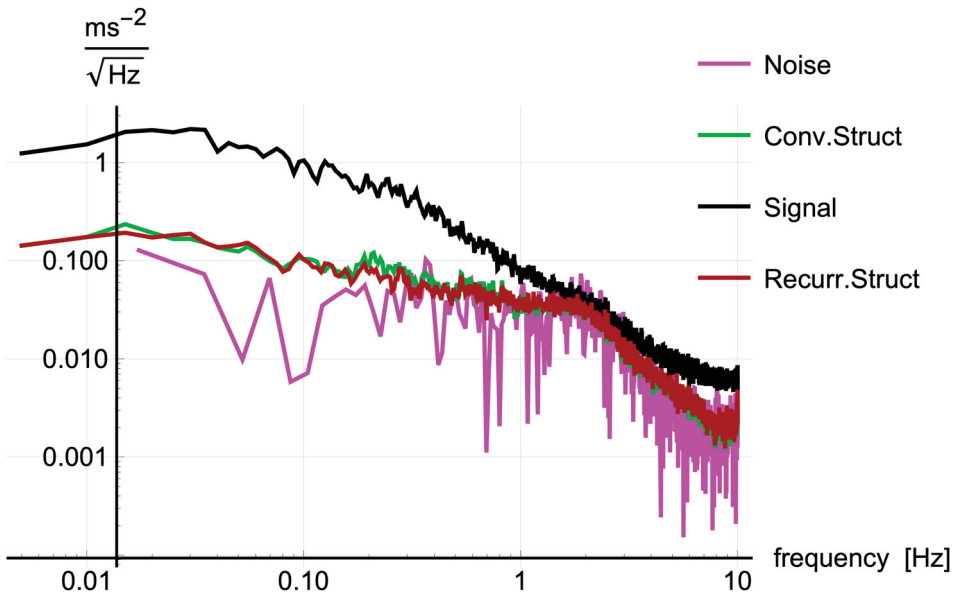
Figure 11. Power spectral density of acceleration measurement noise, convolutional and recurrent structured neural networks fit residuals and measured acceleration signals (training set).
